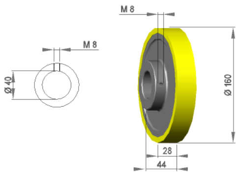
Transportrad TRD 160 / 28 / S70G
