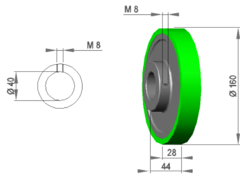
Transportrad TRD 160 / 28 / S90Gr
