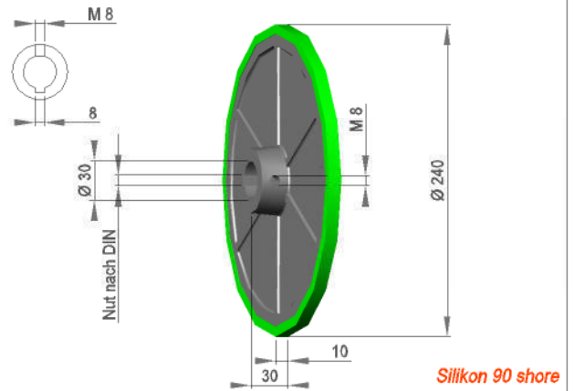
Transportrad TRF 240 / 30 / S90Gr
