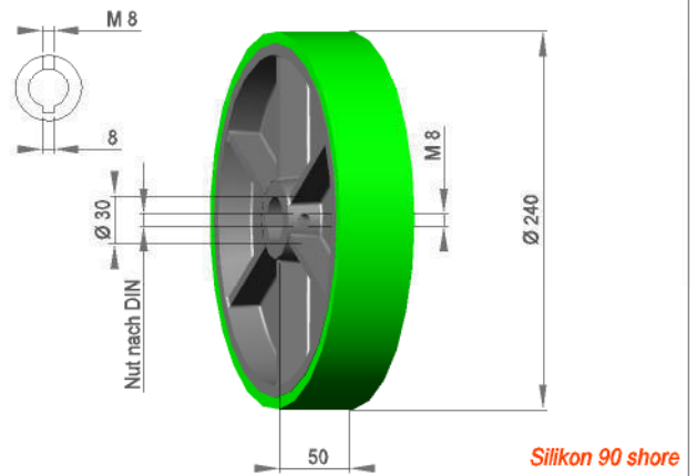
Transportrad TRF 240 / 50 / S90G
