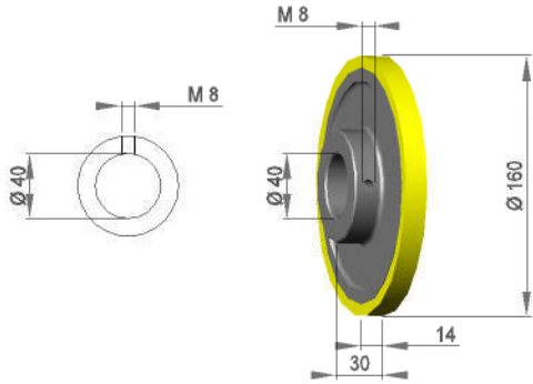
Transportrad TRD 160 / 14 / S70G
