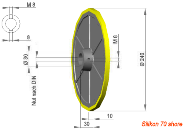
Transportrad TRF 240 / 30 / S70G
