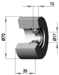
Aluminium
