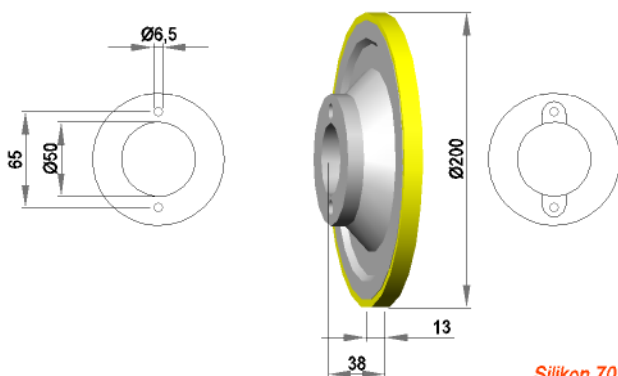
Transportrad TRBA 200 / 13 / S70G
