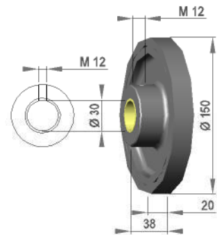
Transportrad TR 150 / 20 / ST
