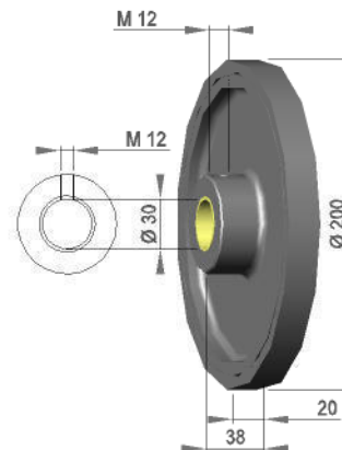
Transportrad TR 200 / 20 / ST
