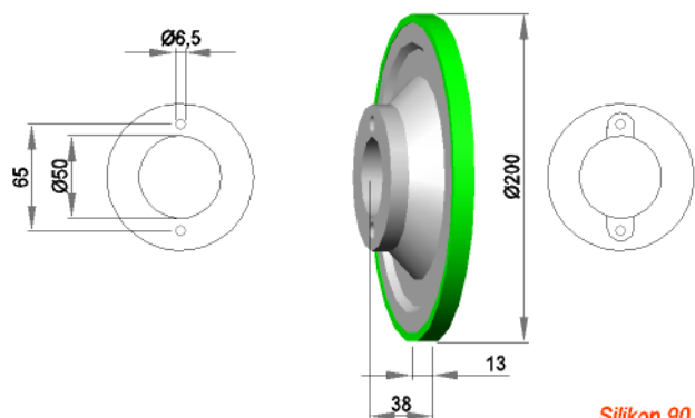
Transportrad TRBA 200 / 13 / S90Gr
