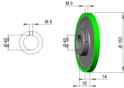
Transportrad TRD 160 / 14 / S90Gr
